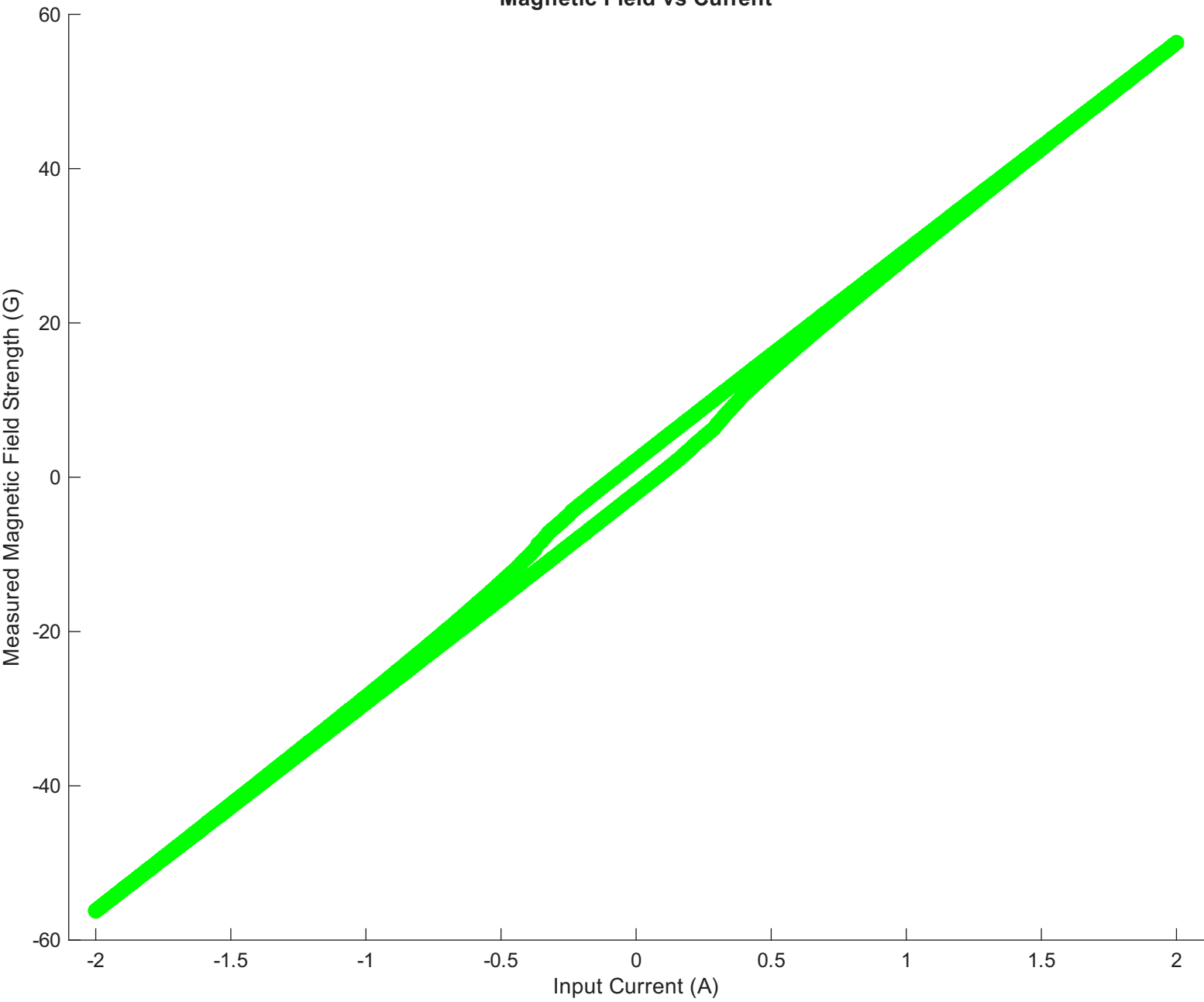
Magnetic Field vs Current
